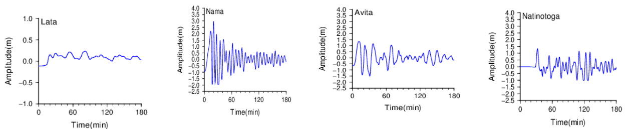
Figure 6 Waveforms at output points (Figure 3 right) for the eastern Solomon study area.
