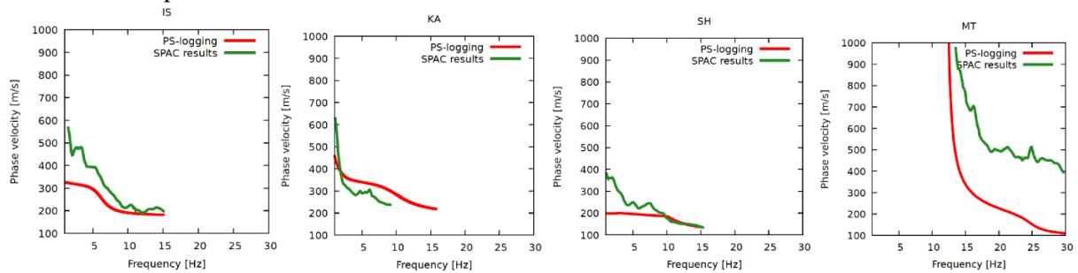
Figure 3. Comparison of the observed phase velocities obtained from SPAC analysis and the theoretical phase velocities obtained from PS-logging data.
