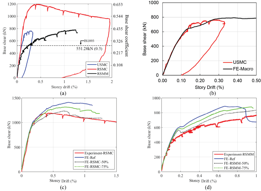
Figure 4. (a) Experimental capacity curves; Comparison of FE generated capacity curve to experimentally obtained capacity curve for (b) USMC (c) RSMC and (d) RSMM.
