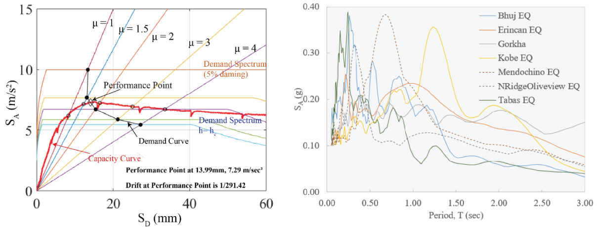
Figure 5. Performance point for PGA of 0.4g of IS 1893-2016 for RSMC house using the CSM method (Left) and Acceleration response spectra for the selected earthquake records at 5% damping (Right).
