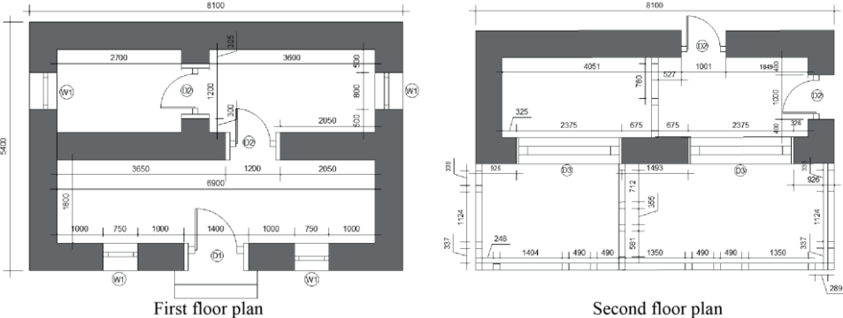
Figure 1. Plan of the target specimen.
