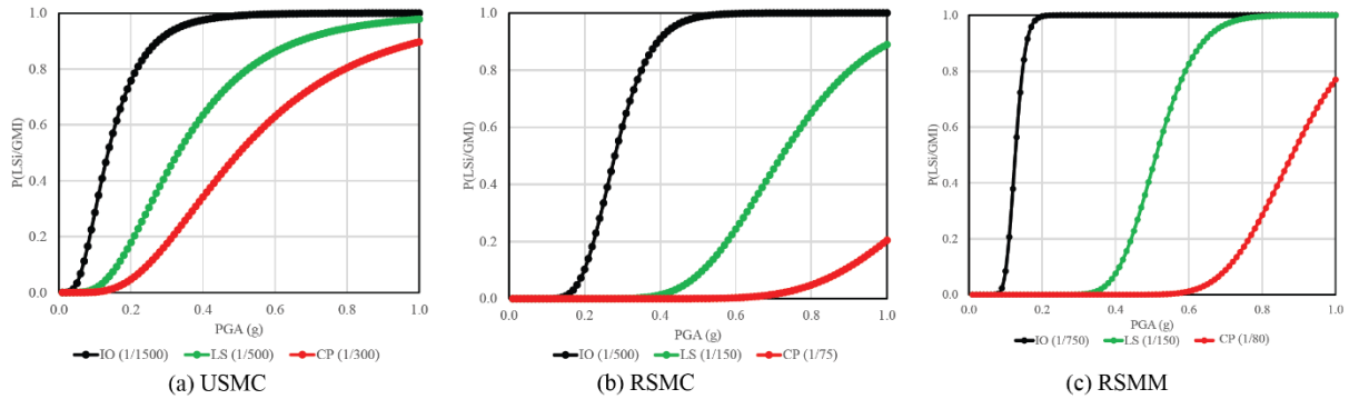
Figure 6. Fragility curves for traditional Bhutanese residential houses.
