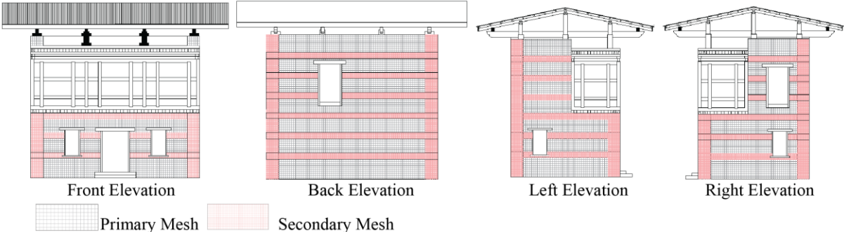
Figure 2. Design of mesh-wrap technique applied to the full-scale specimen.
