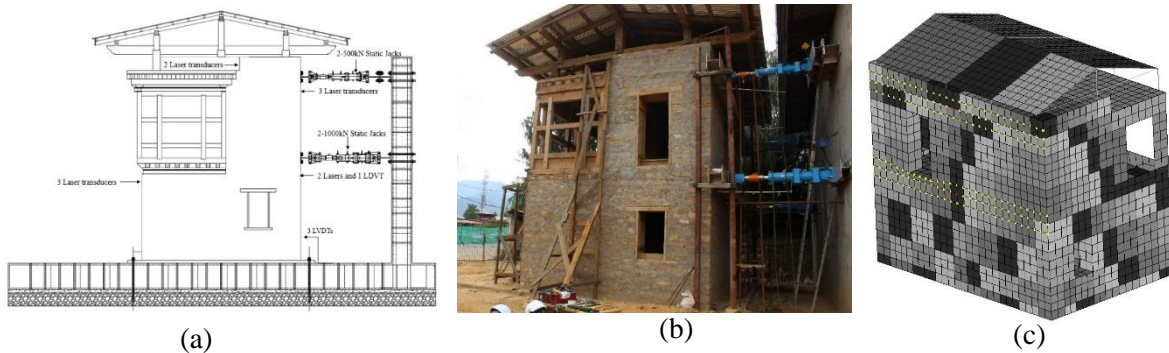
Figure 3. (a) Schematic full-scale quasi-static test setup, (b) Real scenario experimentation setup and (c) FE-numerical model with loading constraints.
