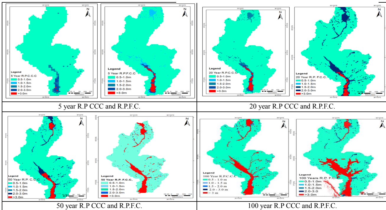
Fig. 6. Inundation maps (Current and Future) for Different Return Periods under the ACCESS model
