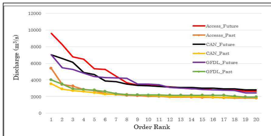
Figure 4: Extreme Daily Discharges (Present and Future Climate)
