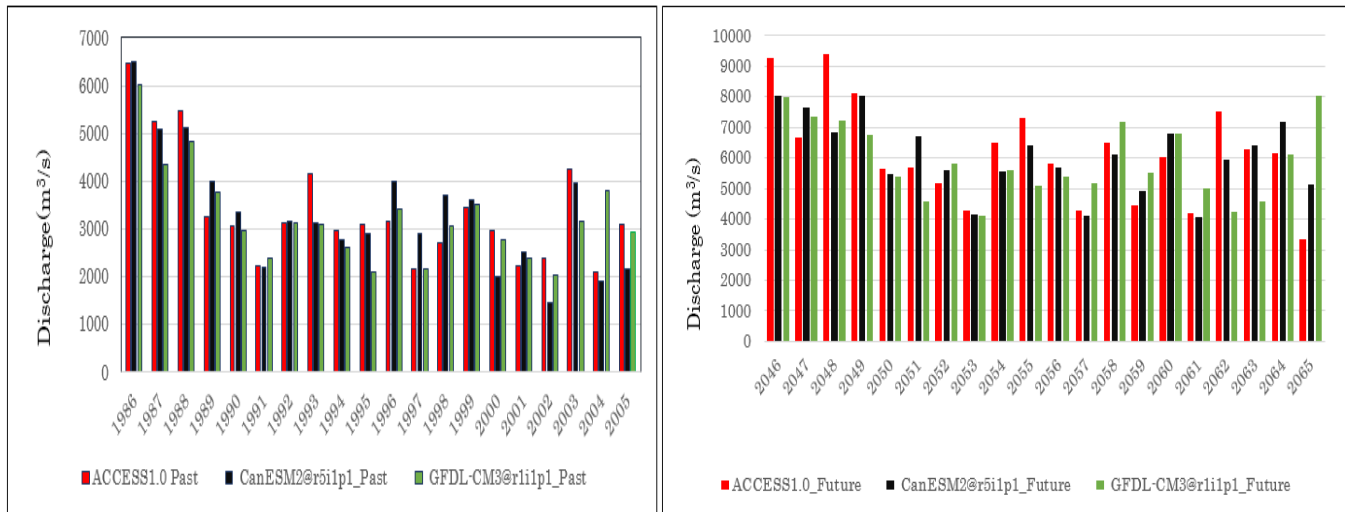
Figure 3: Annual maximum discharge under Current and Future climates at Chiromo station
